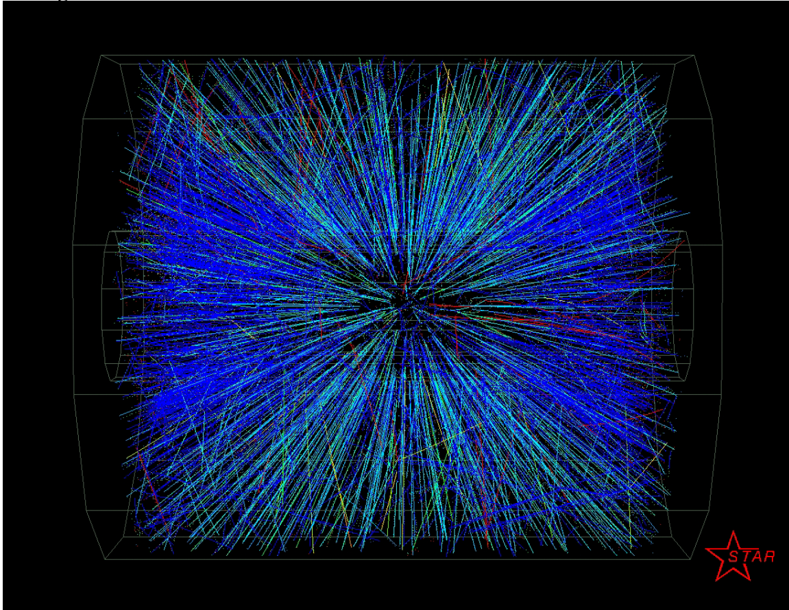
Fig. 9-4. This picture shows a collision between two gold nuclei in the STAR detector at the RHIC accelerator. Each line represents the path of a particle produced in the collision.
